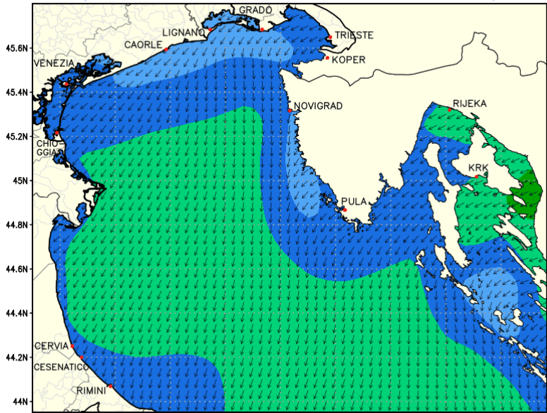
10m Wind [kt]
